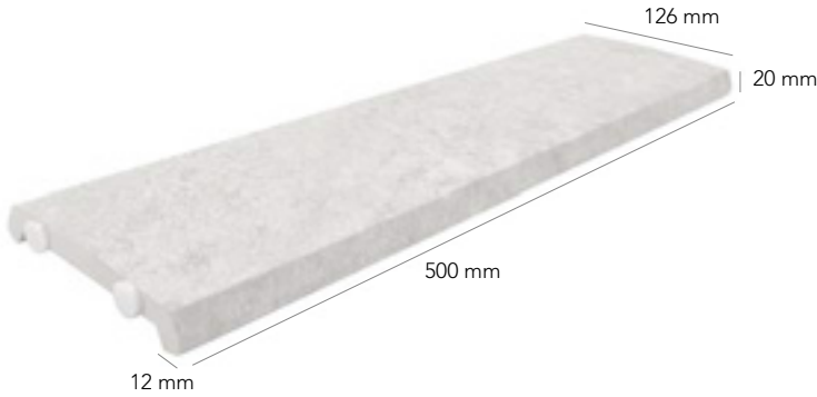
REJILLA OCULTA REGISTRABLE PZ/126 500x126x20 mm (Grosor 12mm)
